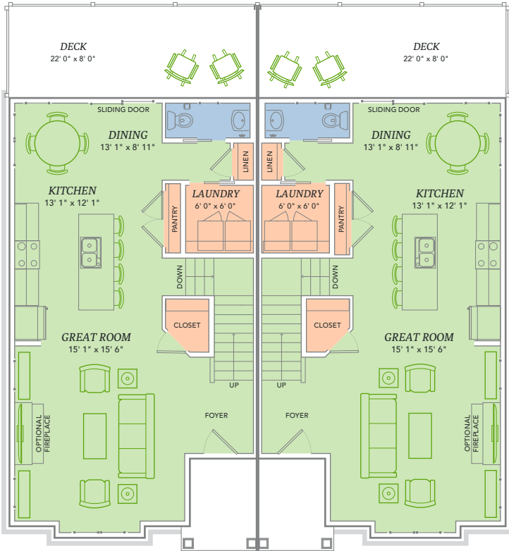
UNIT A First Floor
